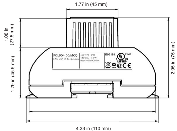
Figure 2: BACnet Communication Module Side View
