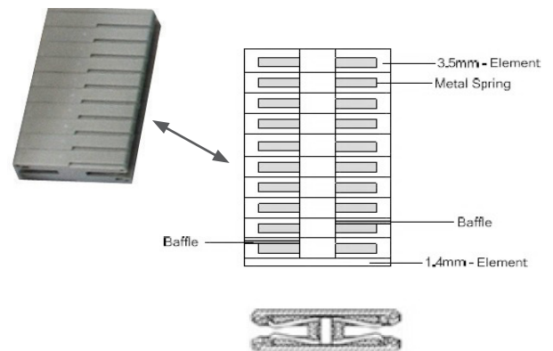
Figure 6: Board-to-Board Connector
