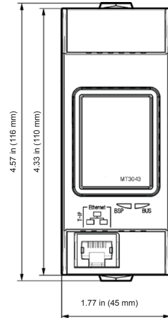
Figure 1: BACnet Communication Module Top View
