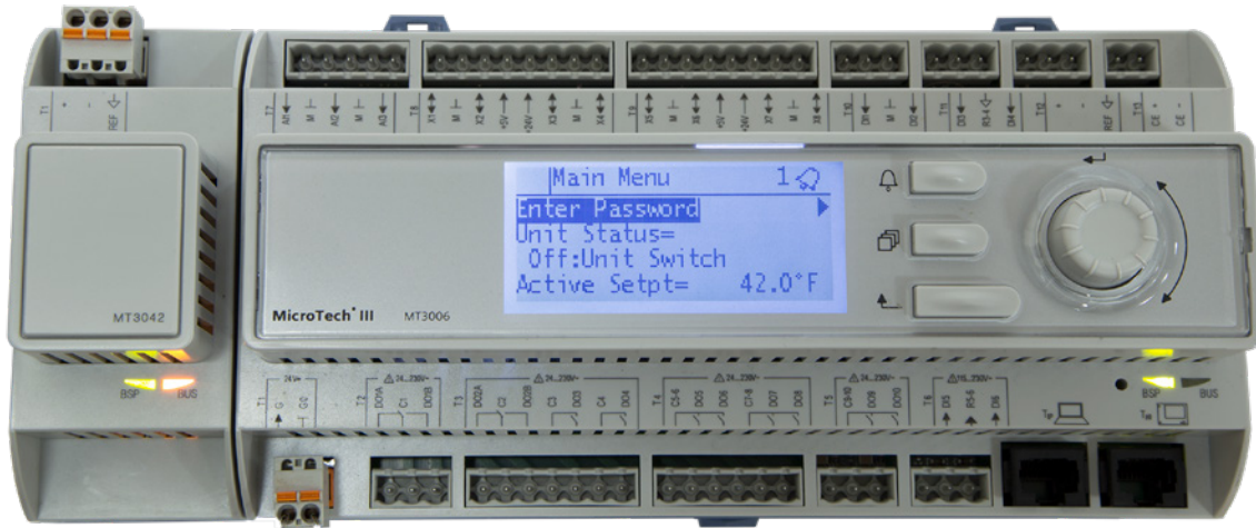
Figure 3: BACnet MS/TP Communication Module Attached to Unit Controller
